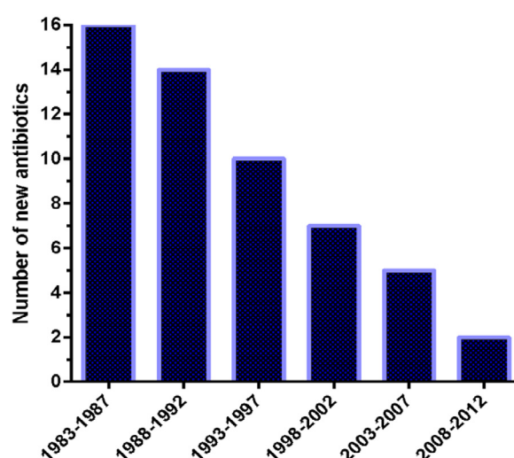
Figure 3: New antibiotics approved in the United States, 1983–2012. The two last antibiotics from new classes were linezolid and daptomycin; both of them target against Gram-positive bacteria. The figure is reproduced from Infectious Diseases Society of America report (21).
