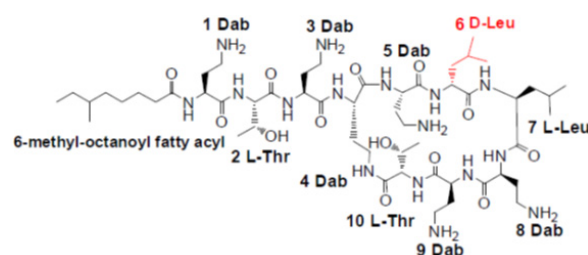
Figure 4: Chemical structure of polymyxin B and colistin. In polymyxin B, D-Phe (phenylalanine) replaces the D-Leu (leucine) marked (red words). Colistin methanesulfonate (CMS) is produced by the reaction of colistin with formaldehyde and sodium bisulphite, which leads to the addition of a sulphomethyl group ( \text{SO}_3\text{CH}_2 ) to the primary amines ( \text{NH}_2 ) of colistin. Dab, \alpha,\gamma -diaminobutyric acid, Thr, threonine. Modified from (22).
